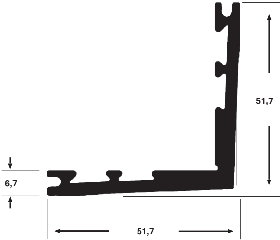
CANTONEIRA L 25
